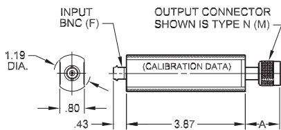
NC346 Coaxial Series Dimensions (inches)
